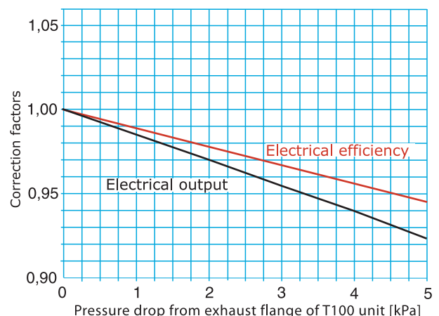
Performance at different exhaust pressure drop
