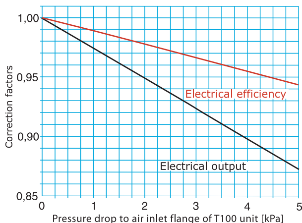
Performance at different inlet pressure drop
